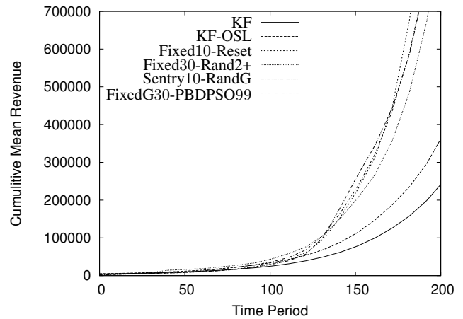
Fig. 4. Mean cumulative revenue earned with demand parameters changing with time with overall upward trend
