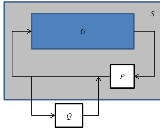
Fig. 5. After designing P , the plant as seen by Q is given by S = (I - PG)^{-1} .
