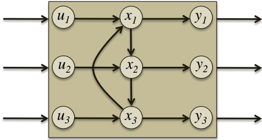
Fig. 1: System with a ring structure, given by Equations (3) and (4).
